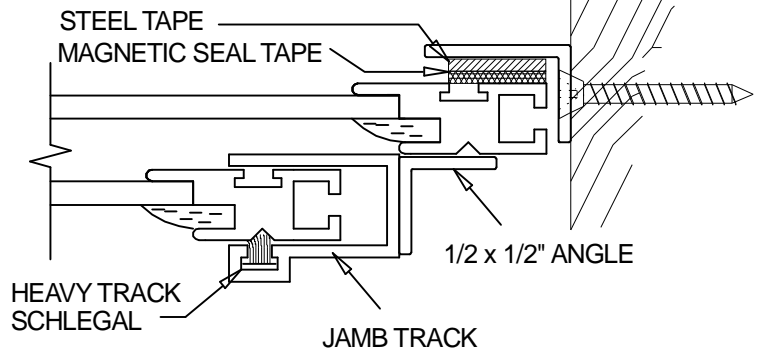
2 JAMB DETAIL SCALE: FULL
