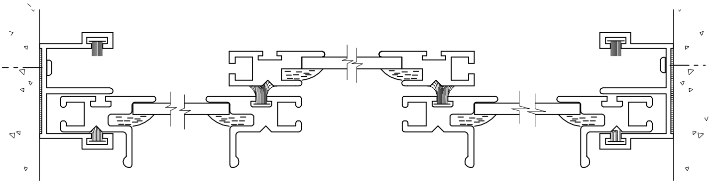
4 MEETING RAIL DETAIL SCALE: FULL
